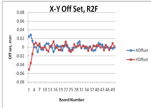
Figure 11. X-Y off set correction for R2F
