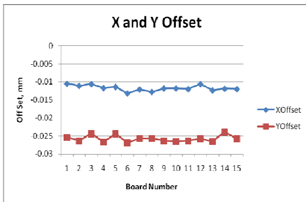
Figure 6. Gage study result for SE300 SPI system
