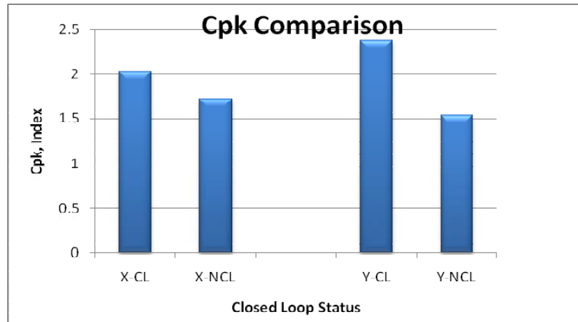
Figure 13. Cpk comparison for with/without closed loop
