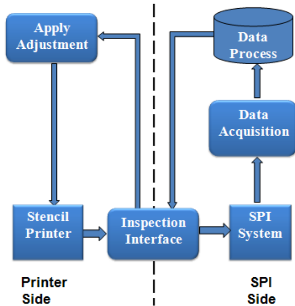
Figure 4. Control scheme
