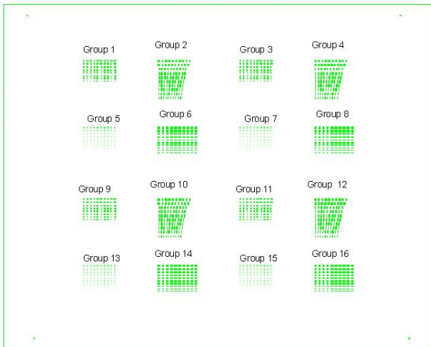
Figure 10. Stencil layout
