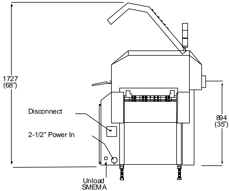
Bravo 8105 Unload End View
