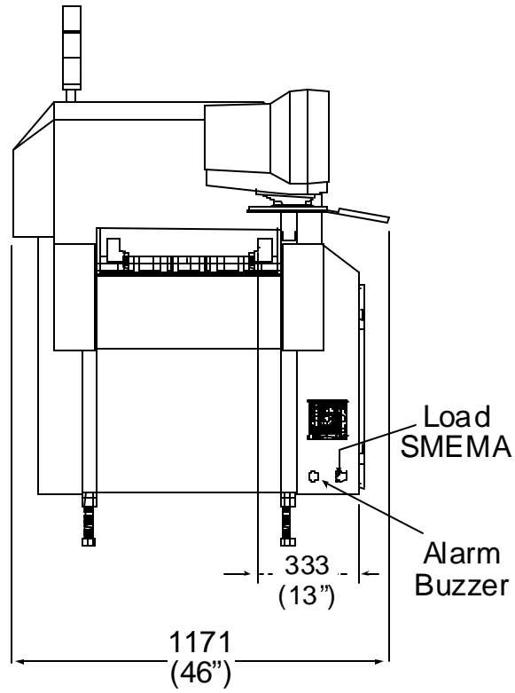
Bravo 8105 Load End View
